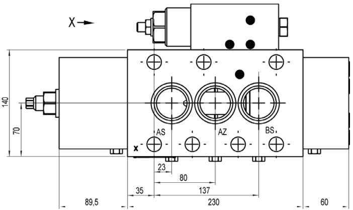
1000 l/min Version
