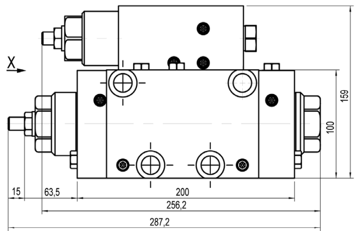
400 l/min Version
