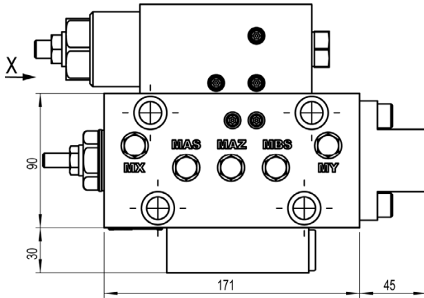
250 l/min Version
