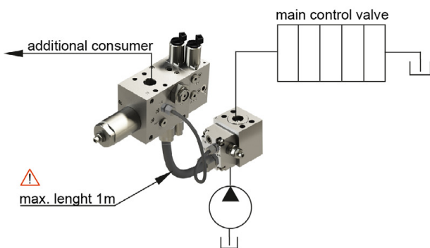
Installation: Open-Center Hydraulic System
