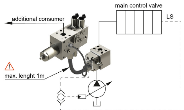
Installation: Closed-Center Hydraulic System
